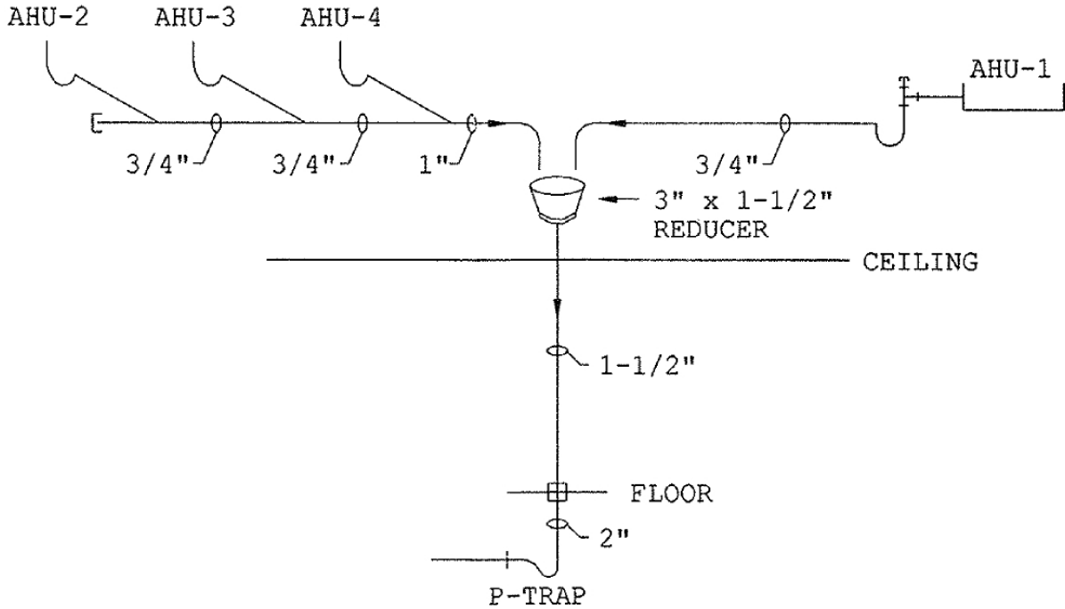
CONDENSATE DRAIN SCHEMATIC
