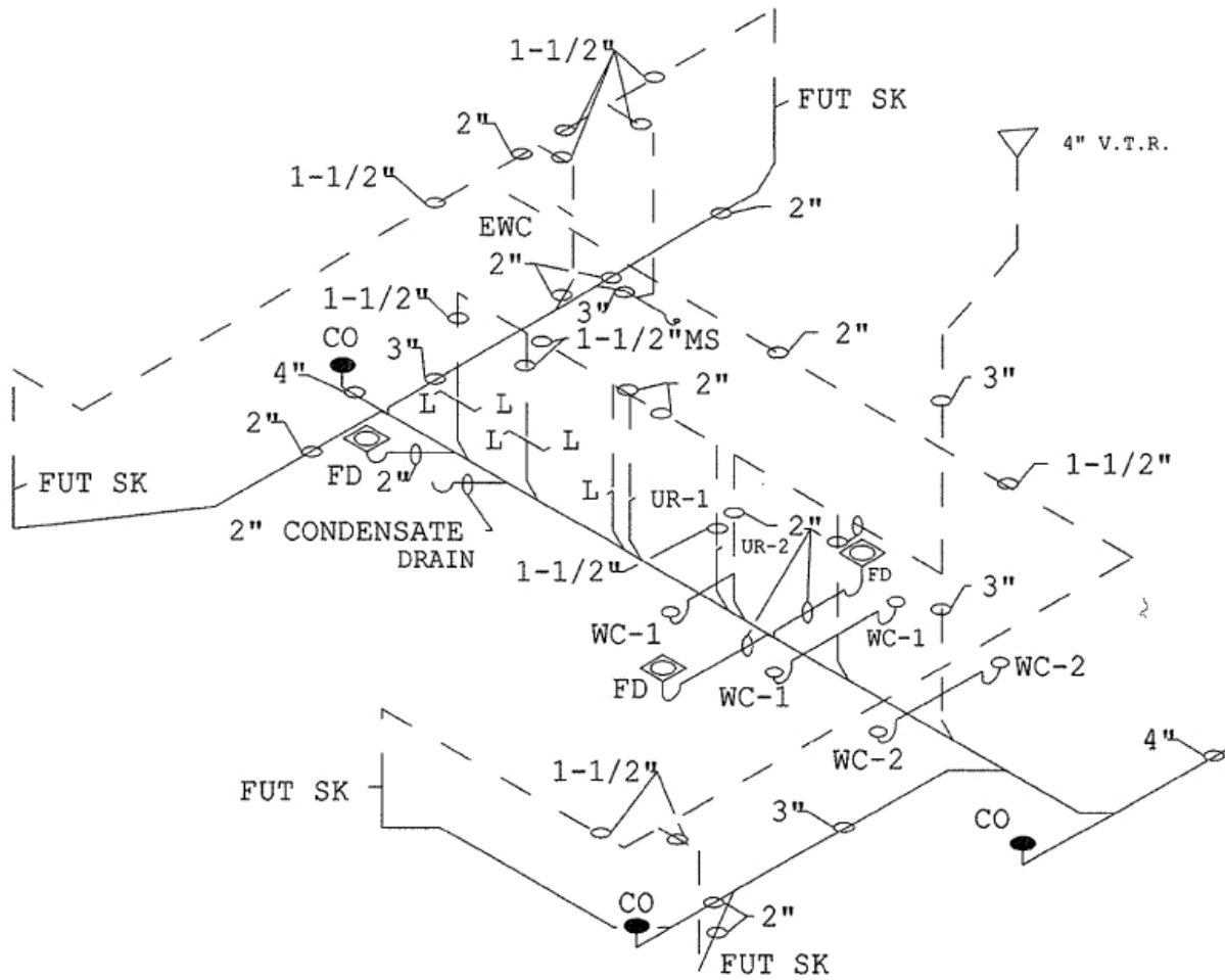
SANITARY/VENT ISOMETRIC
